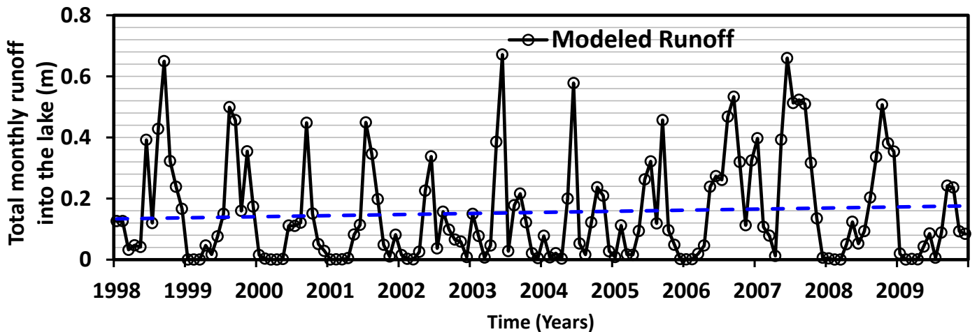
Figure 16: Modeled total monthly runoff over Lake Turkana basin, 1998–2009. Blue line indicates statistical trend.
