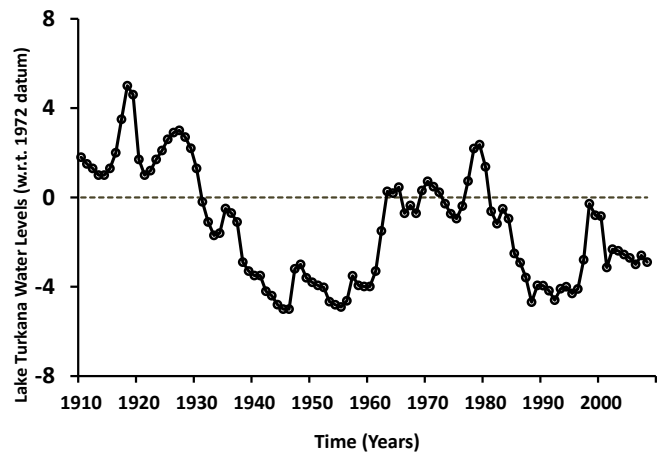
Figure 2: Lake Turkana water levels in the 20th century. Source: KMFRI, Kenya
