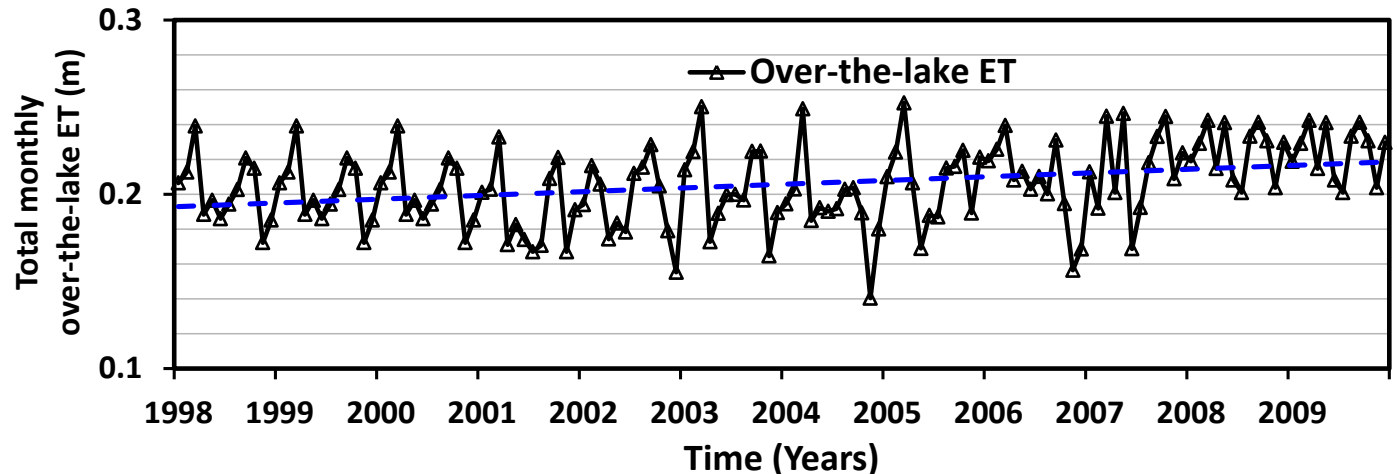
Figure 17: Total monthly evapotranspiration over Lake Turkana, 1998–2009. Blue line indicates statistical trend.
