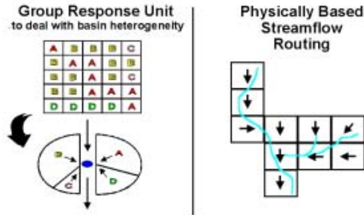
Fig. 5.4-1 Group response unit and runoff routing concept (Donald, 1992)
