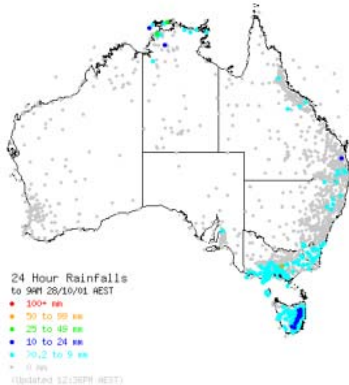
Fig. 5.3-1 Twenty-four hour rainfalls in Australia (Source: FWSBM, 2001)
