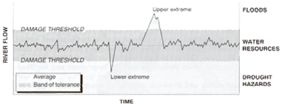
Fig. 2.2-2 Sensitivity to flood hazard expressed in relation to the variability of river discharge and the degree of socio-economic tolerance at a site (Source: Modified from Hewitt and Burton, 1971)
